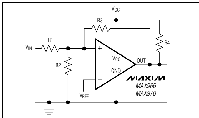
Figure 4. External Hysteresis
