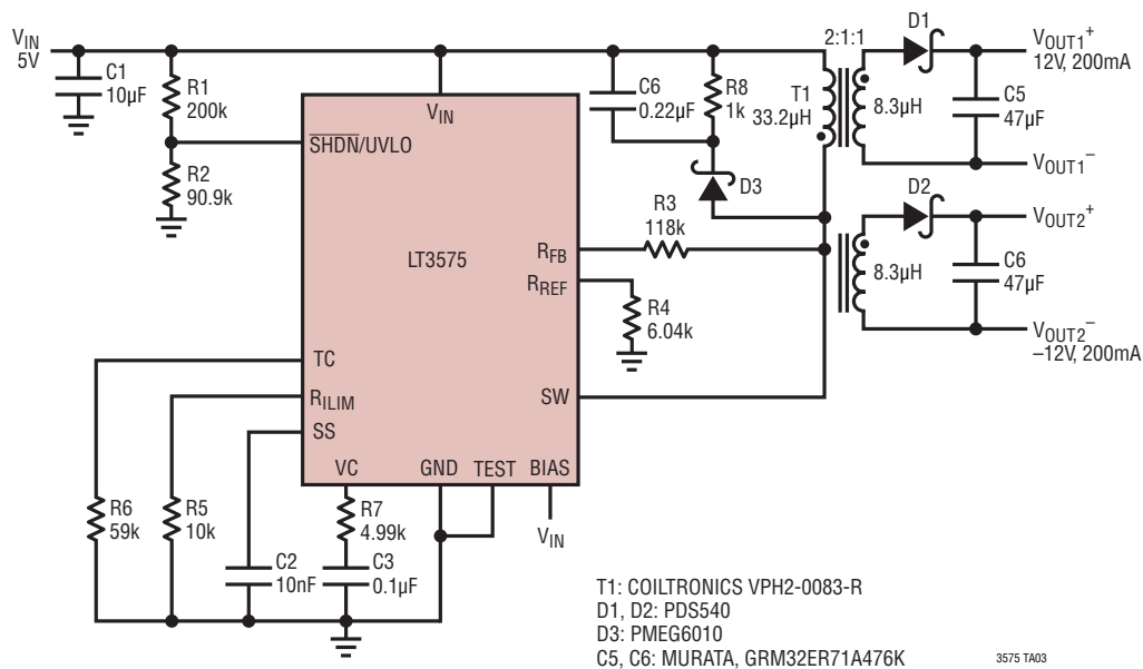
\pm 12V Isolated Flyback Converter
