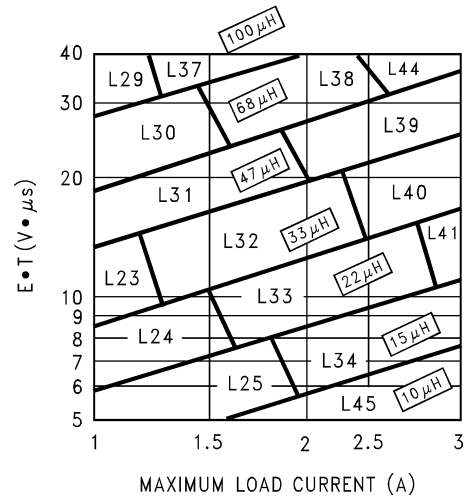
Figure 7-5. LM2670 – Adjustable
