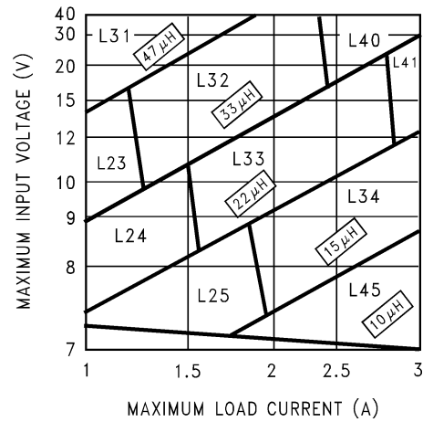
Figure 7-3. LM2670 – 5 V
