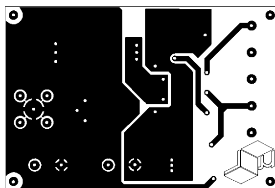
Figure 7. Bottom Layer
