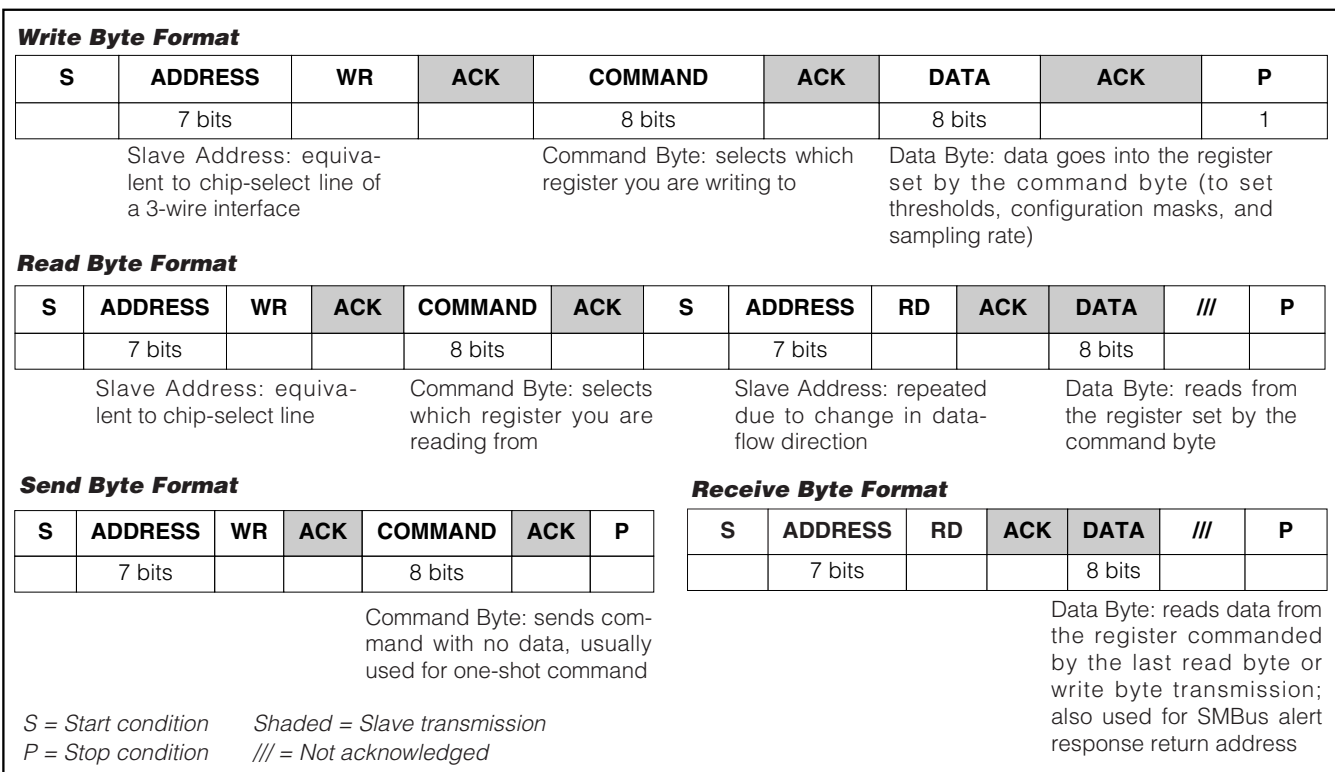
Figure 2. SMBus Protocols
