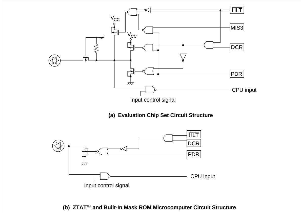
Figure 27 NMOS Intermediate-Voltage Open Drain Pin Circuits
