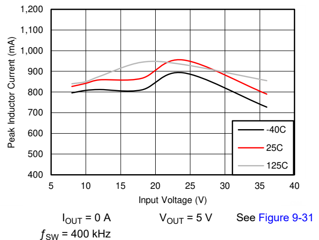
Figure 7-6. I_{PEAK-MIN}
