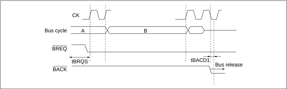
Figure 8.43 When \overline{\text{BREQ}} is Input without Satisfying \text{tBRQS}
