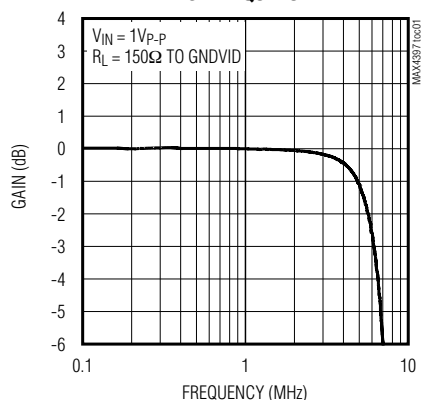
R/G/B VIDEO LARGE-SIGNAL BANDWIDTH vs. FREQUENCY
