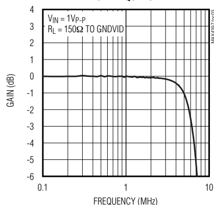
Y VIDEO LARGE-SIGNAL BANDWIDTH vs. FREQUENCY
