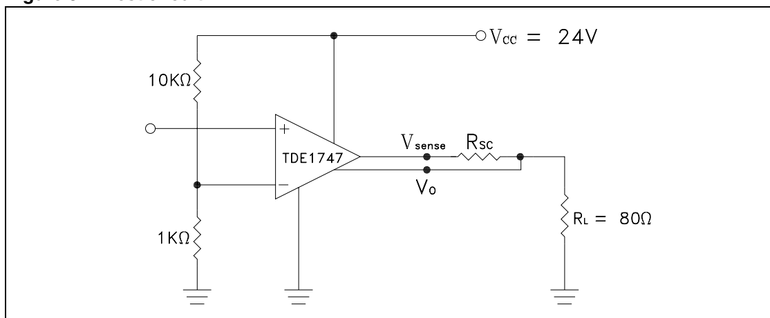
Figure 3. Test circuit
