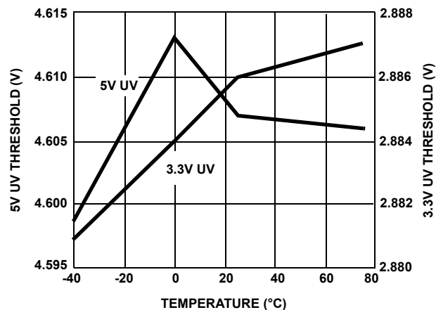
FIGURE 4. 3.3V/5V UV THRESHOLD
