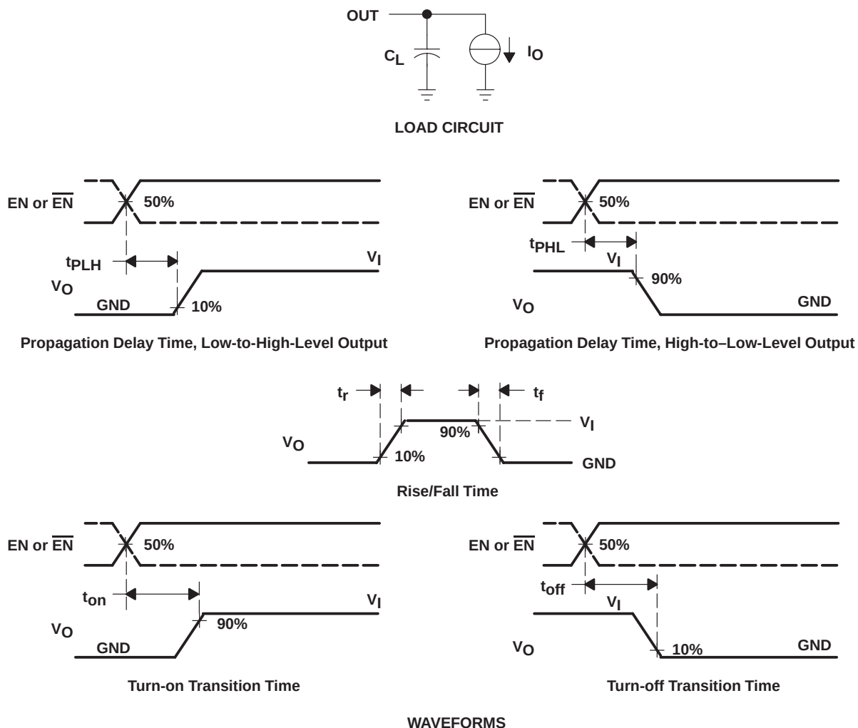
Figure 3. Test Circuit and Voltage Waveforms
