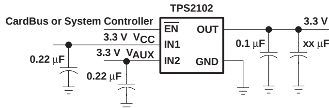
Figure 24. Typical Application
