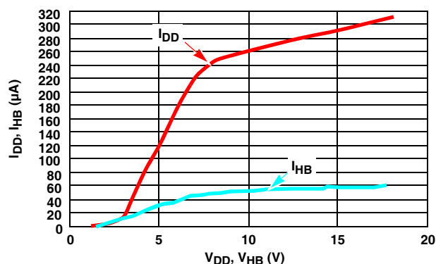
FIGURE 20. ISL2111 QUIESCENT CURRENT vs VOLTAGE
