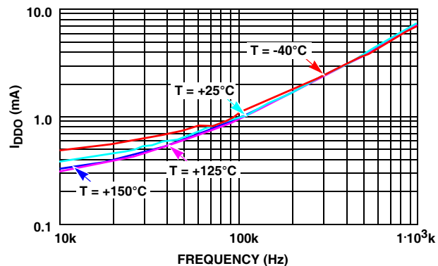
FIGURE 6. ISL2111 I DD OPERATING CURRENT vs FREQUENCY
