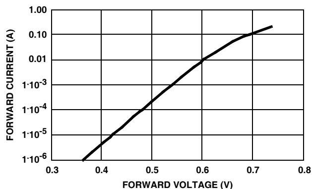
FIGURE 21. BOOTSTRAP DIODE I-V CHARACTERISTICS
