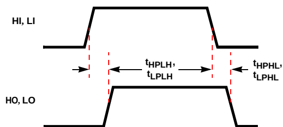
FIGURE 3. PROPAGATION DELAYS
