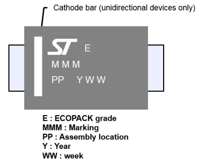
Figure 19. SMA marking
