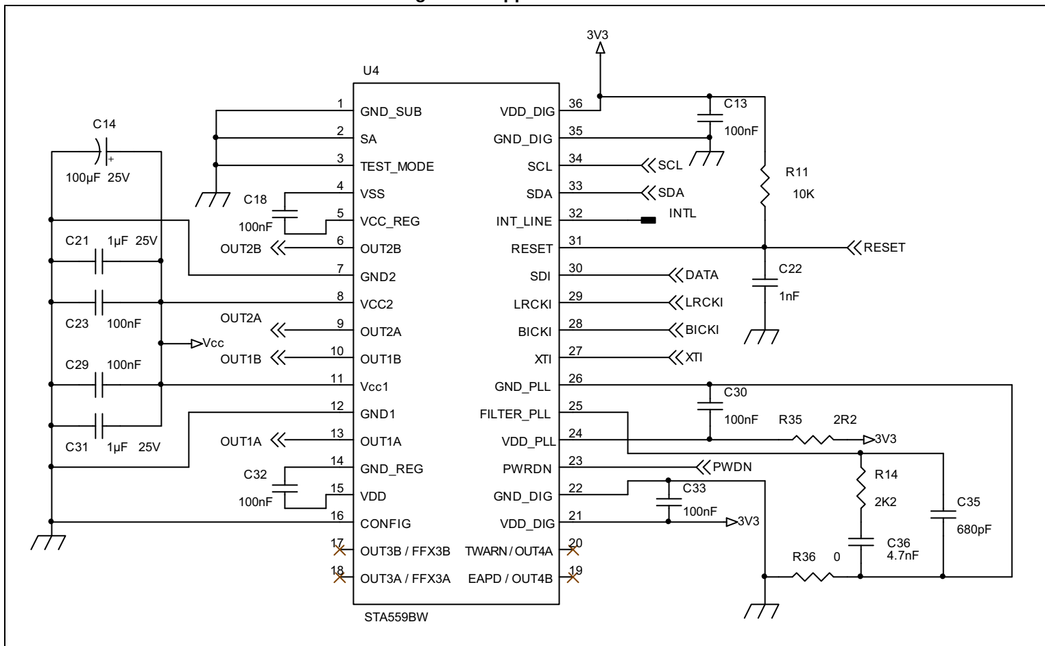
Figure 19. Applications circuit
