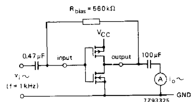
Fig. 7 Test set-up for measuring forward transconductance g_{fs} = di_o/dv_i at v_o is constant (see also graph Fig. 8); MR = \text{LOW} .
