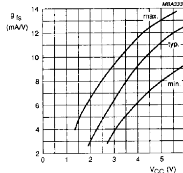
Fig. 8 Typical forward transconductance g_{fs} as a function of the supply voltage V_{CC} at T_{amb} = 25^\circ\text{C} .
