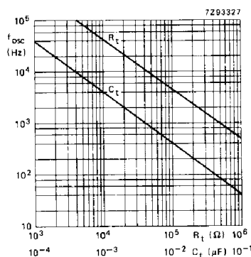
Fig. 9 RC oscillator frequency as a function of R_t and C_t at V_{CC} = 2.0 to 6.0 V; T_{amb} = 25^\circ\text{C} .
