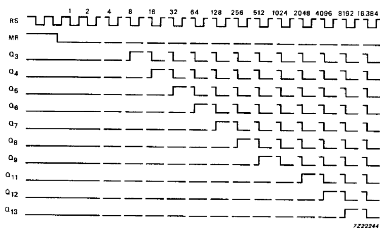
Fig. 6 Timing diagram.
