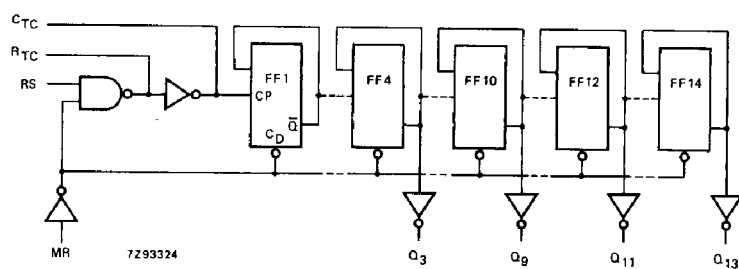
Fig. 5 Logic diagram.
