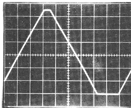
FIGURE 9A. OUTPUT WAVEFORM WITH INPUT SIGNAL RAMPING (2V/DIV., 500 \mu S/DIV.)
