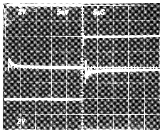
Top Trace: Output Signal; 2V/Div., 5 \mu s/Div. Center Trace: Difference Signal; 5mV/Div., 5 \mu s/Div. Bottom Trace: Input Signal; 2V/Div., 5 \mu s/Div.
