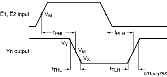
Fig. 5. Input (E1, E2) to output (Yn) propagation delays and output transition times
