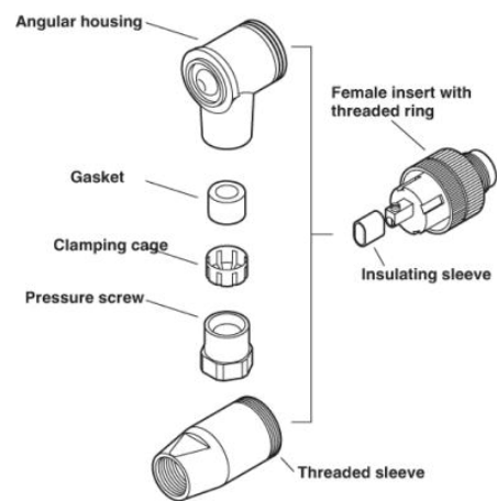
Male/Female M12
