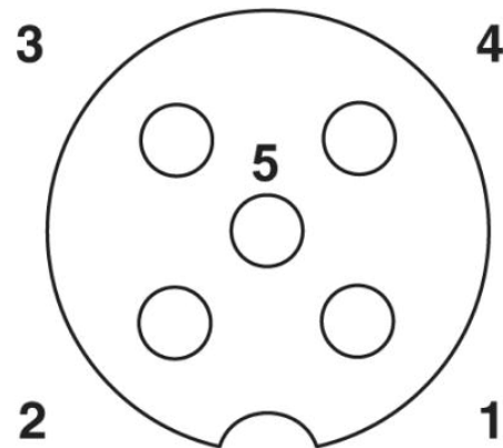
Male/Female M12
