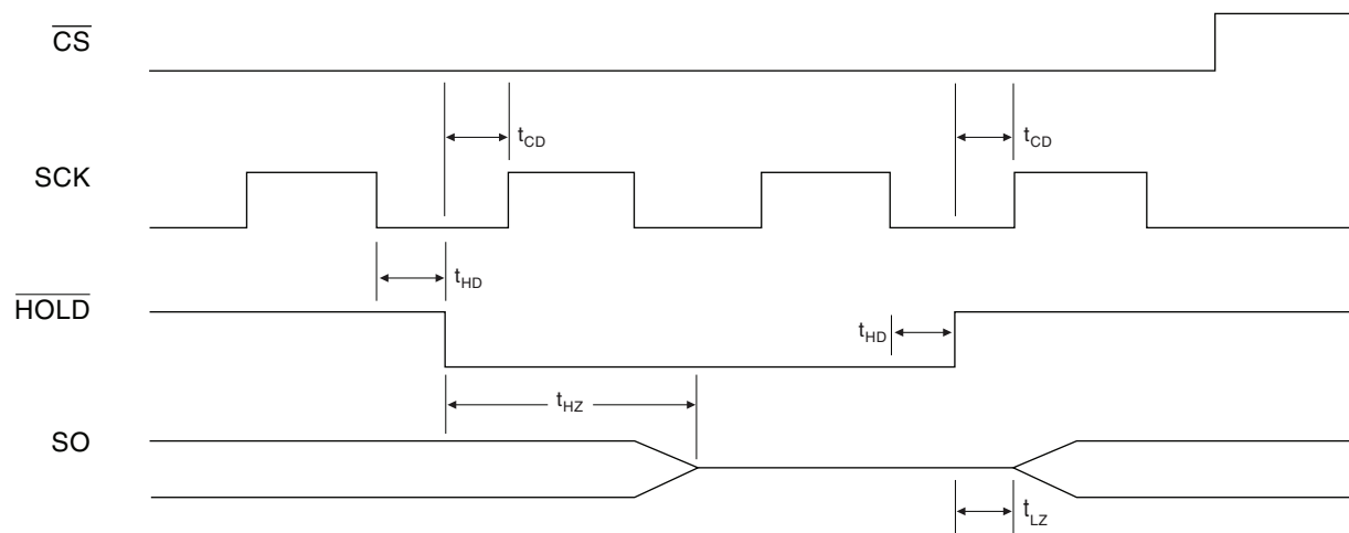
Figure 4-8. \overline{\text{HOLD}} Timing
