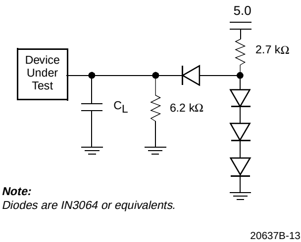
Figure 8. Test Setup
