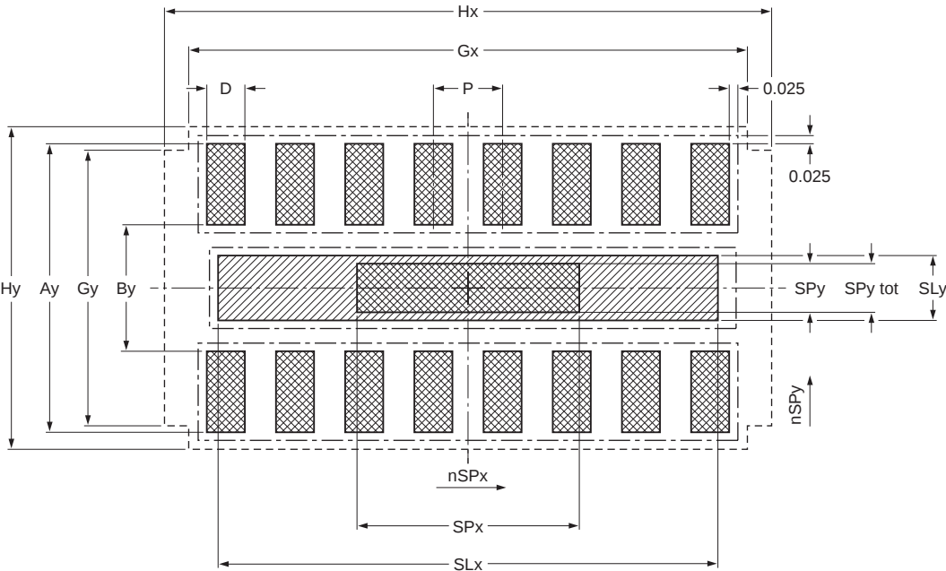
Generic footprint pattern Refer to the package outline drawing for actual layout
