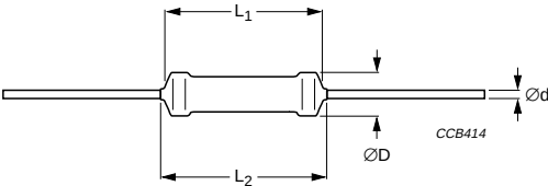
Fig.15 Outline.
