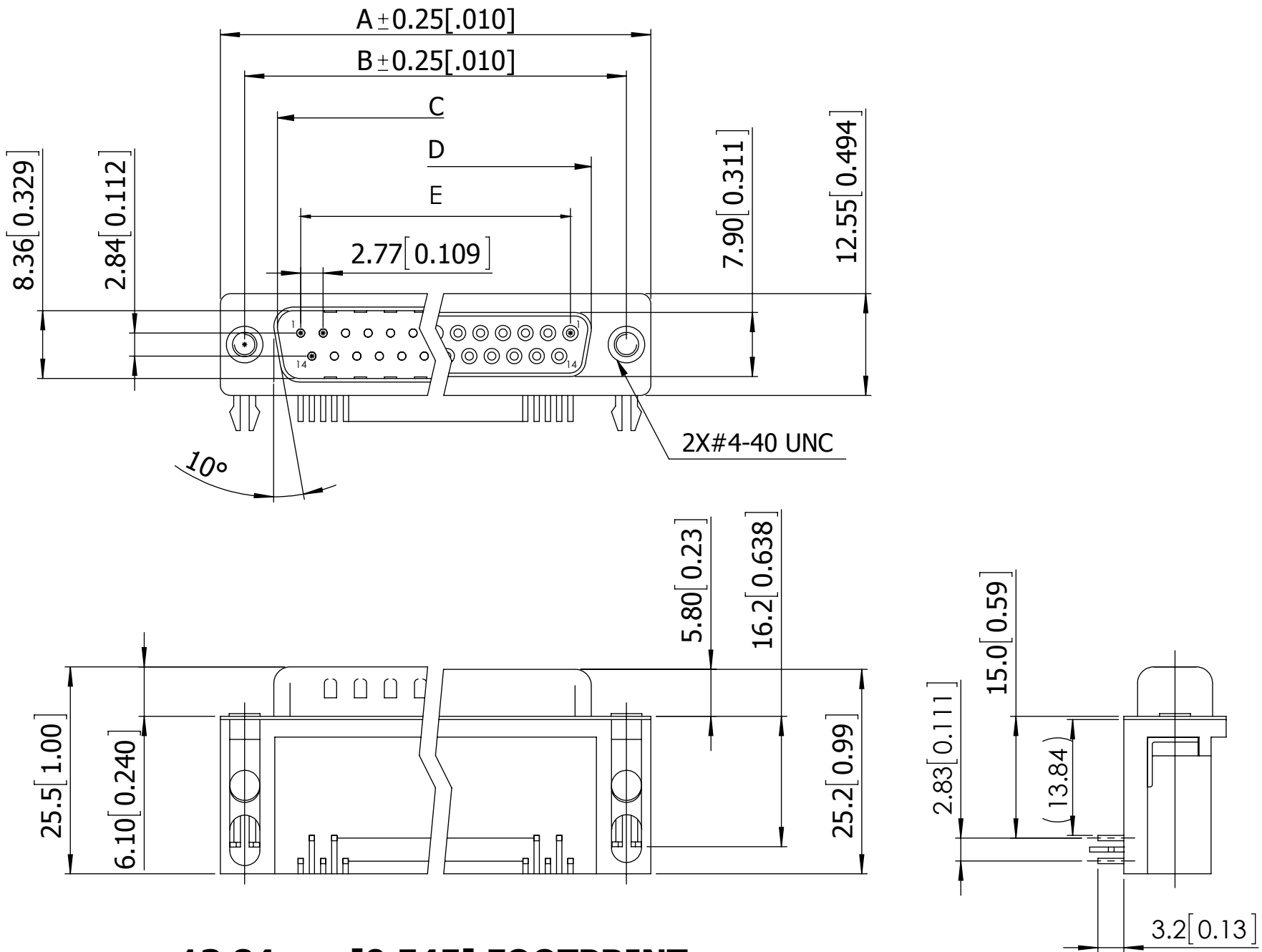
13.84mm [0.545] FOOTPRINT ( PN EXAMPLE: SDS107-PRP2-M09-SN13-13 )
