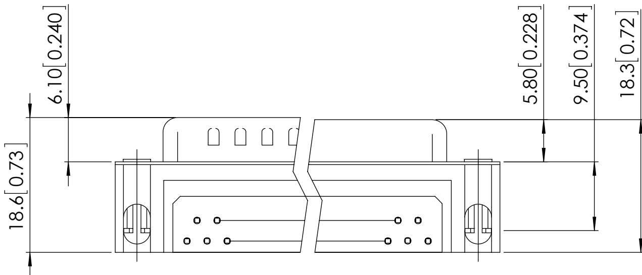
7.2mm [0.28] FOOTPRINT
