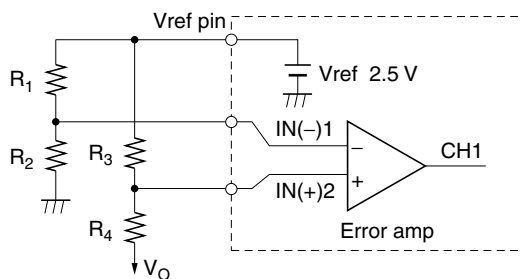
Figure 2.2 Inverting Output
