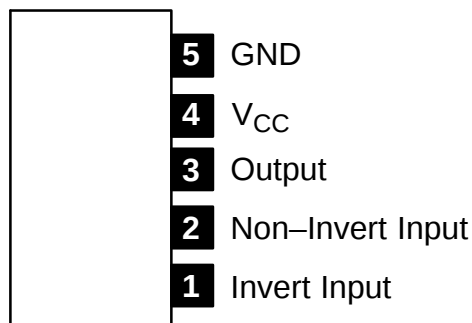
Pin Connection Diagram (Front View)
