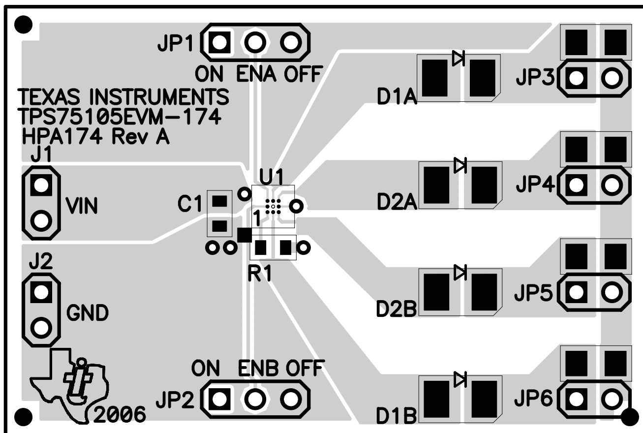
Figure 1. Assembly Layer
