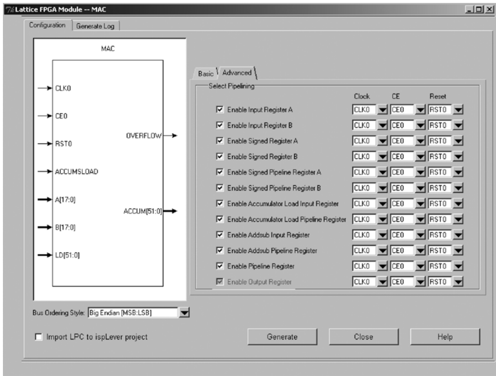
Figure 14-5. MAC Mode Advanced Set-up
