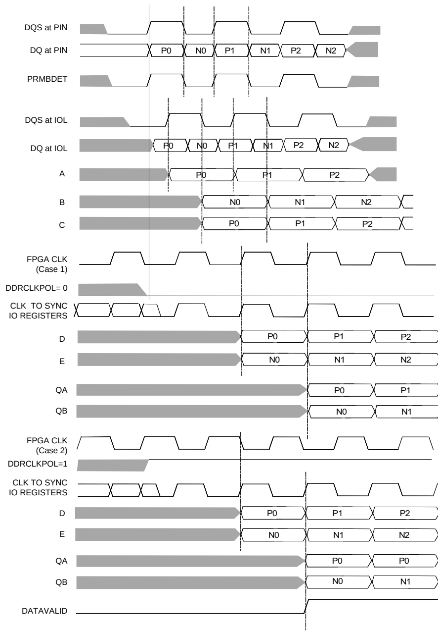
Figure 12-22. Read Data Transfer When Using IDDRMFX1A
