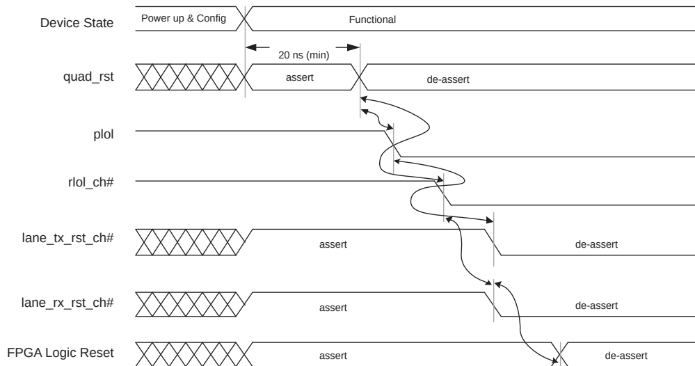
Figure 8-44. Reset Sequence
