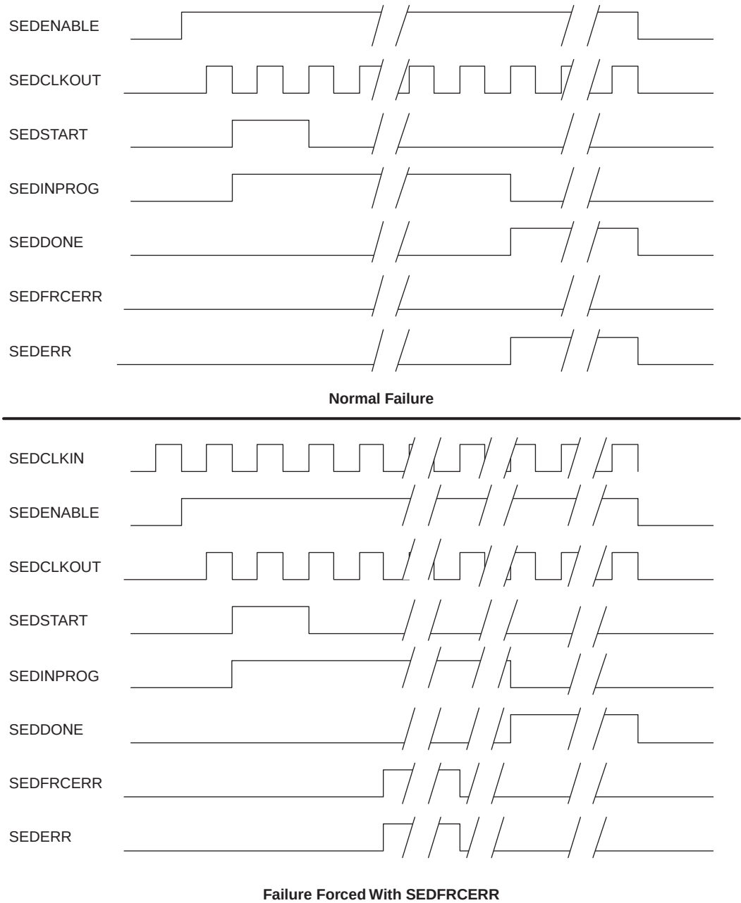
Figure 17-3. Timing Diagram
