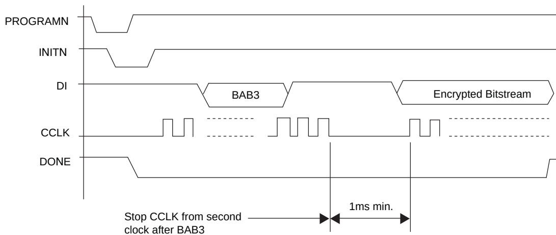
Figure 16-2. CCLK Timing
