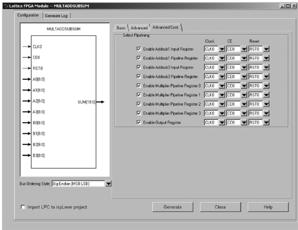
Figure 14-10. MULTADDSUBSUM Mode Advance
