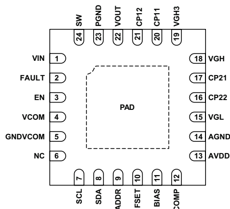
Package ES, 24-Pin QFN Pinouts
