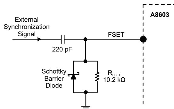
Figure 10: Countermeasure to Prevent External Sync Signal Stuck-at-Low Fault
