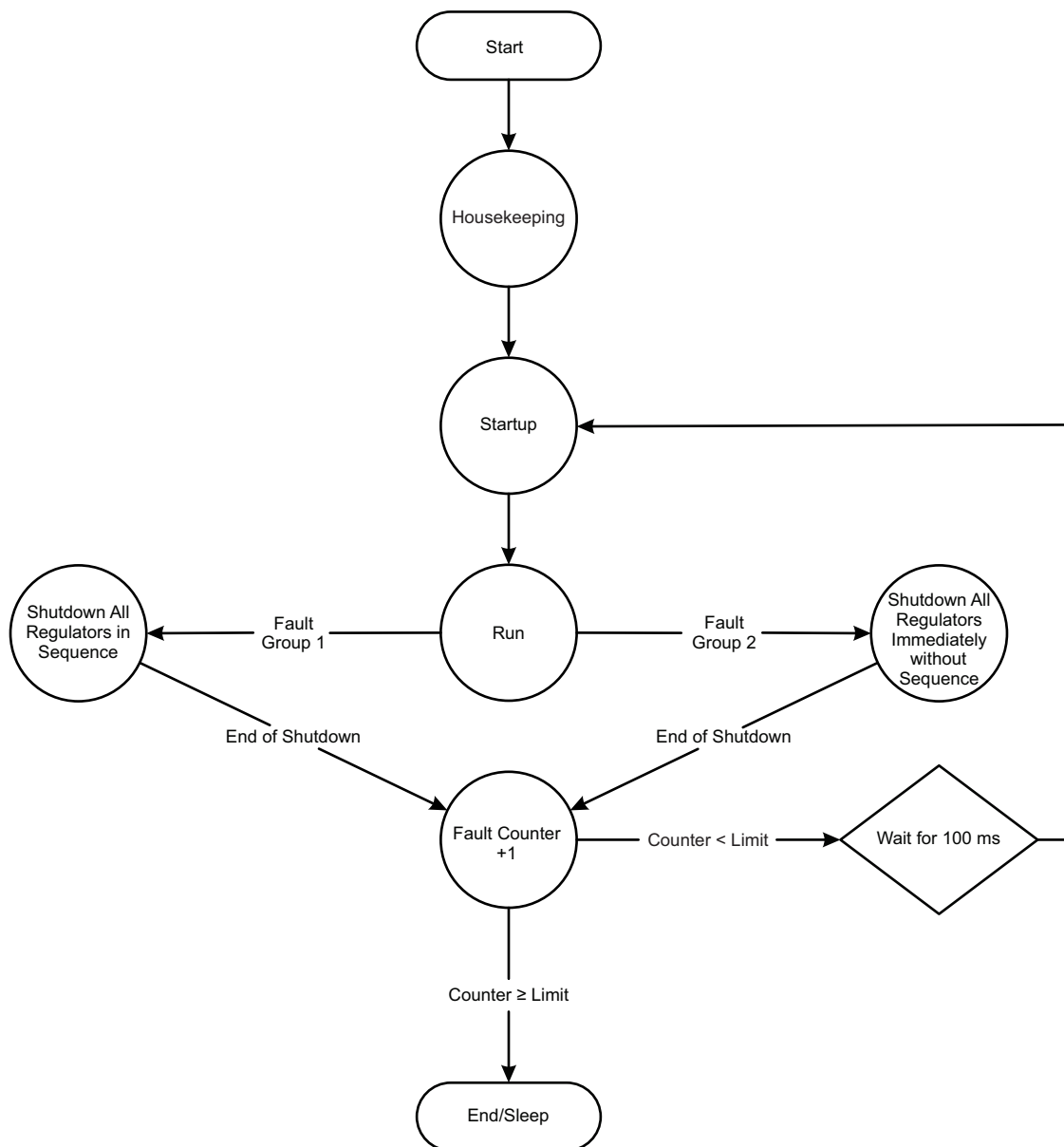
Figure 18: Fault-Retry Counter
