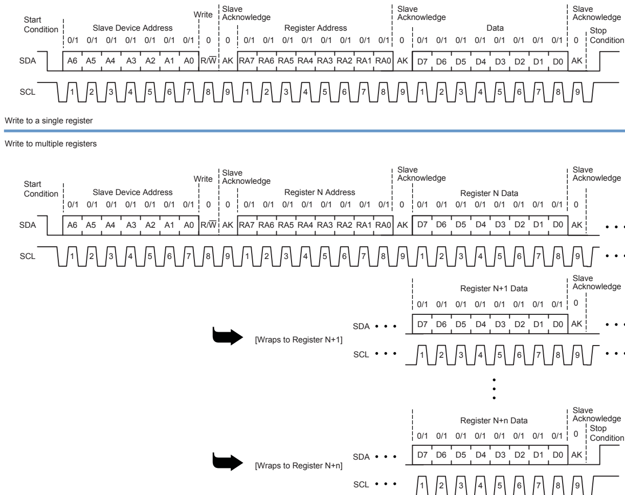
Figure A-3. Writing to single and to multiple registers
