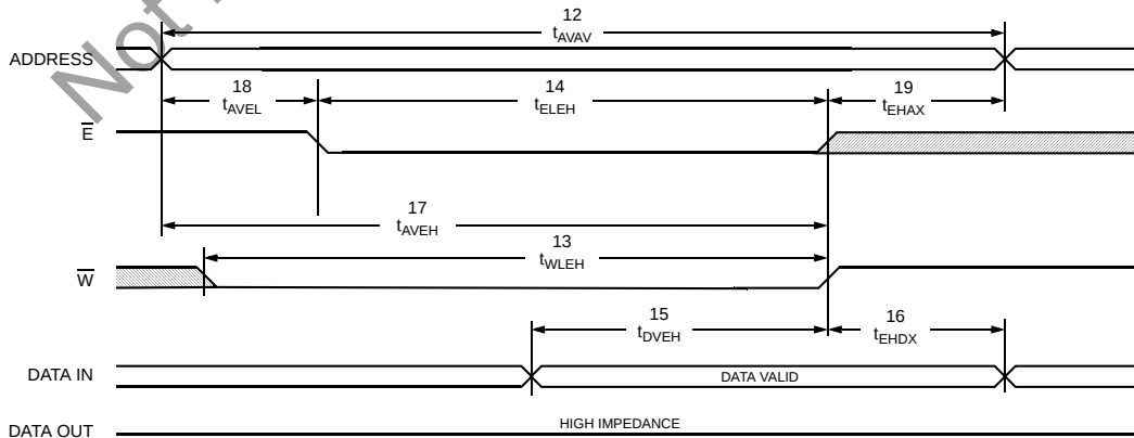
Figure 7. SRAM Write Cycle 2: \overline{E} Controlled [10, 11]
