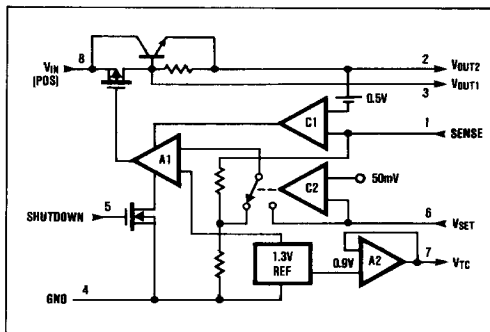
Figure 1. MAX663 Positive Regulator, Block Diagram
