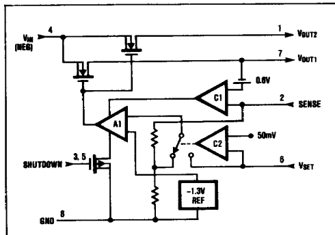
Figure 2. MAX664 Negative Regulator, Block Diagram
