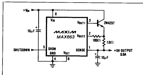
Figure 9. Positive Regulator With Boosted Output, Current Limit, and Low I_Q Shutdown
