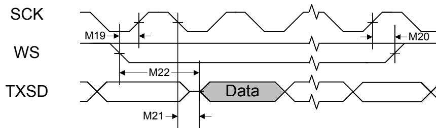
Figure 26-19. I 2 S Slave Mode Transmit Timing
