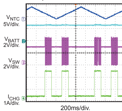
NTC Control,
