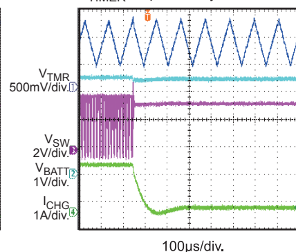
Timer Out
