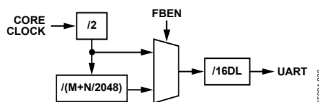
Figure 37 : Fractional Divider Baud Rate generation
