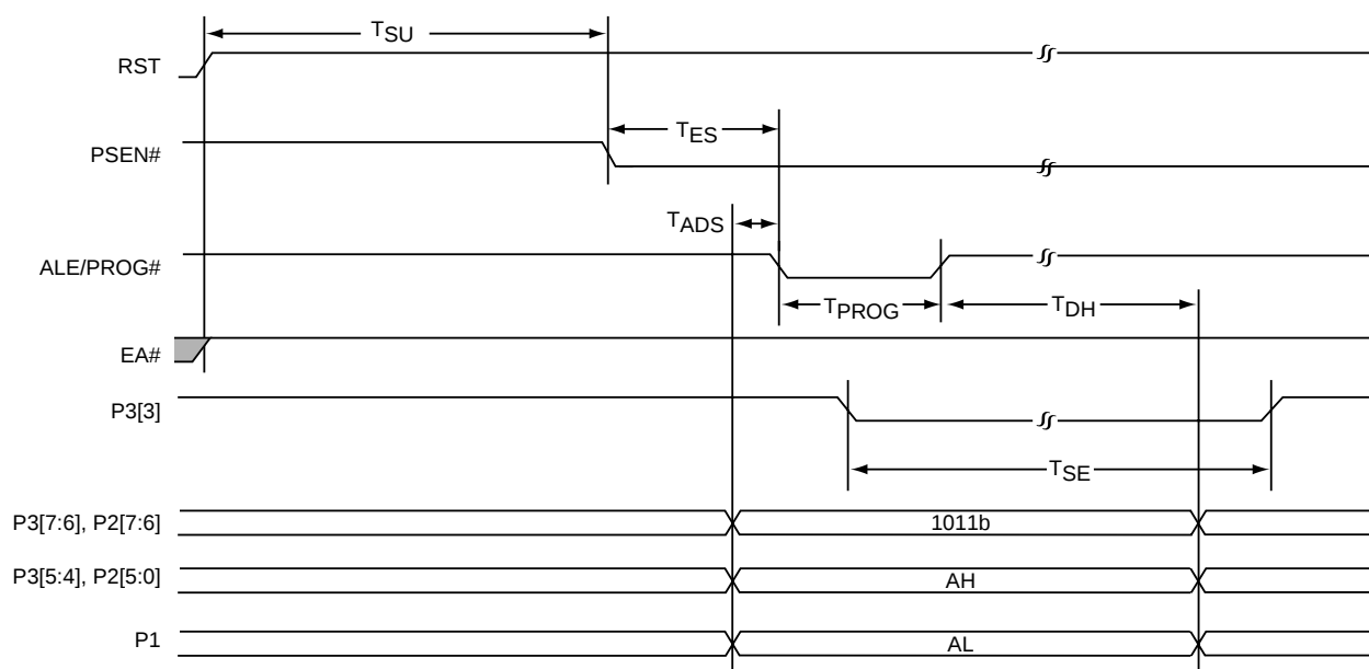
FIGURE 12-15: SECTOR-ERASE
