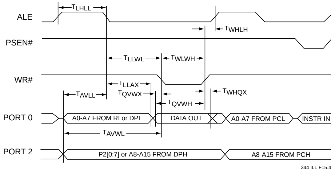
FIGURE 12-3: EXTERNAL DATA MEMORY WRITE CYCLE
