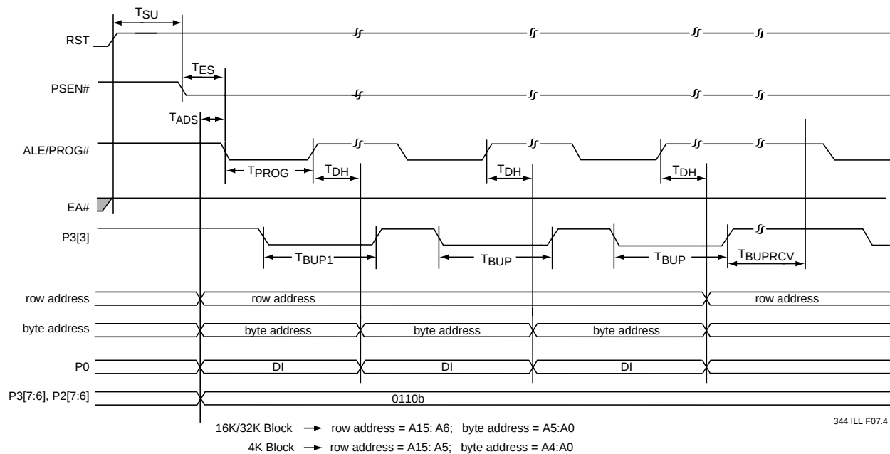
FIGURE 12-17: BURST-PROGRAM
