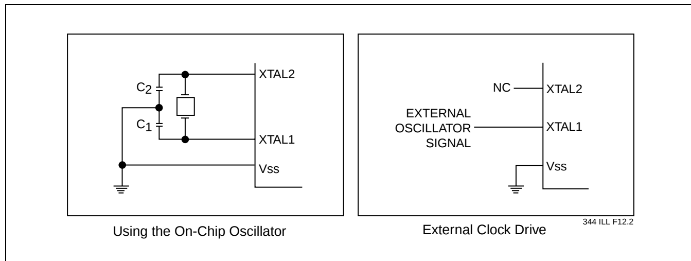
FIGURE 11-1: OSCILLATOR CHARACTERISTICS
