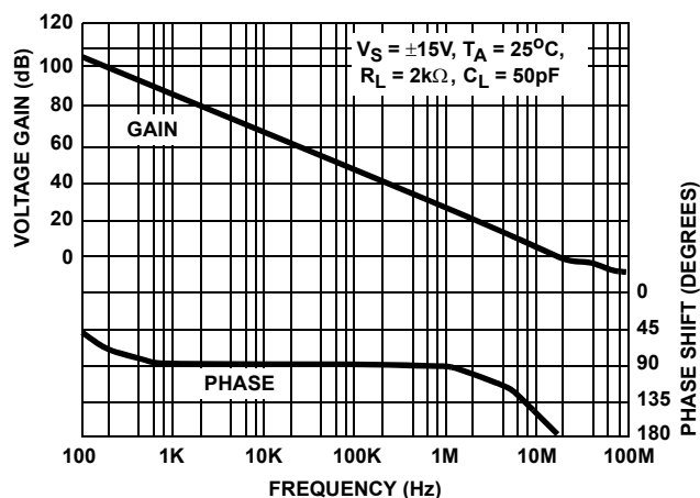
FIGURE 22. OPEN LOOP GAIN vs FREQUENCY
