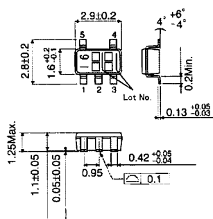
BU4S584G2(SSOP5)(UNIT:[mm])
