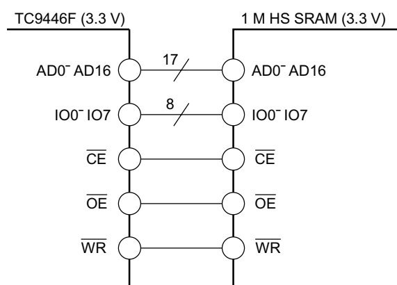
Figure 21 Example of Connection of External SRAM
