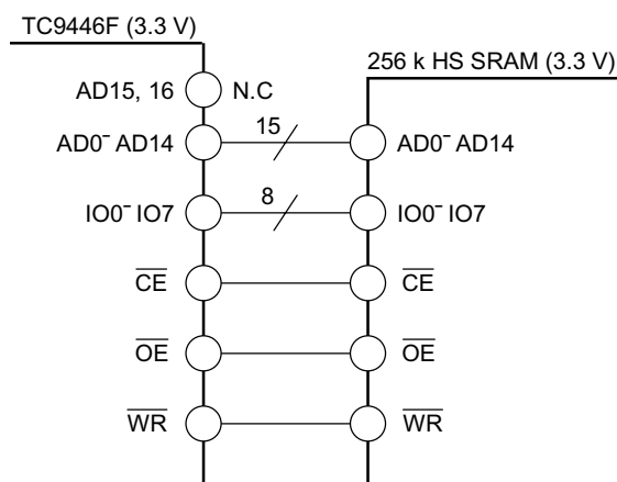
Example of High-speed 256 k SRAM connection
