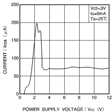
Fig.3 I_{cc} vs. V_{cc}
