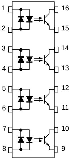
TLP292-4
