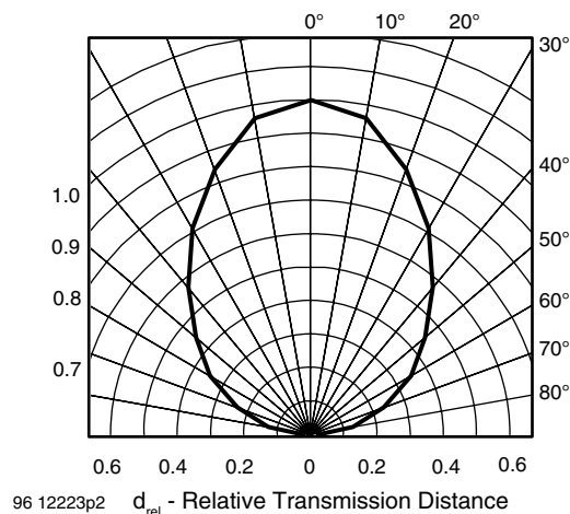
Fig. 12 - Horizontal Directivity
