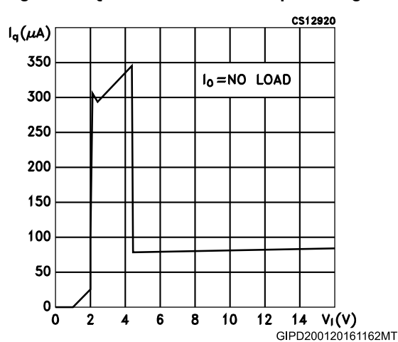
Figure 12: Quiescent current vs input voltage
