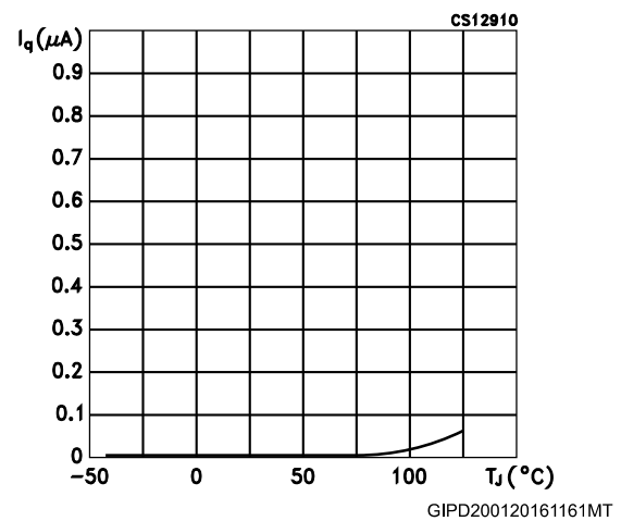
Figure 11: Off mode quiescent current vs temperature
