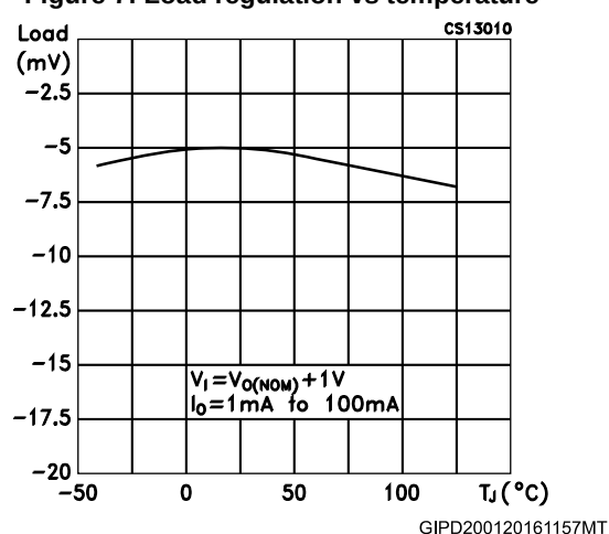
Figure 7: Load regulation vs temperature
