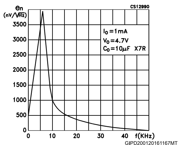
Figure 17: Noise voltage vs frequency
