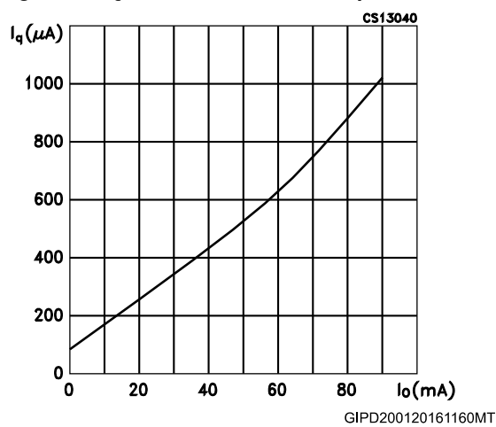
Figure 10: Quiescent current vs output current
