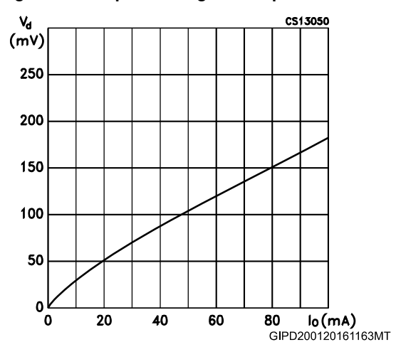
Figure 13: Dropout voltage vs output current
