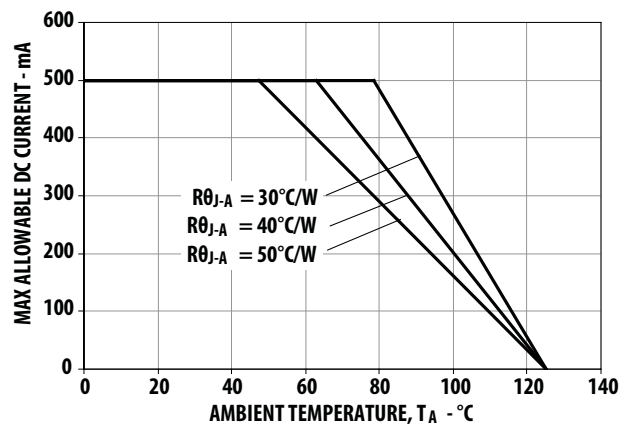
Figure 10. Maximum Forward Current vs. Ambient Temperature. Derated based on T_{JMAX} = 125^{\circ}\text{C} , R_{\theta J-A} = 30^{\circ}\text{C/W} , 40^{\circ}\text{C/W} and 50^{\circ}\text{C/W} .
