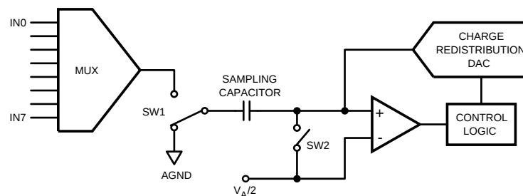
Figure 35. ADC088S022 in Hold Mode
