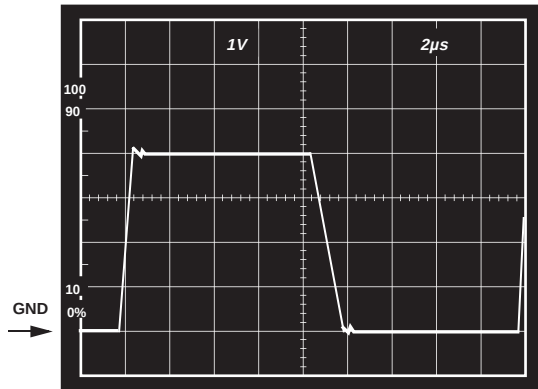
Figure 31. V_S = +5\text{ V} , 0\text{ V} ; Unity Gain Follower Response to 0\text{ V} to 4\text{ V} Step
