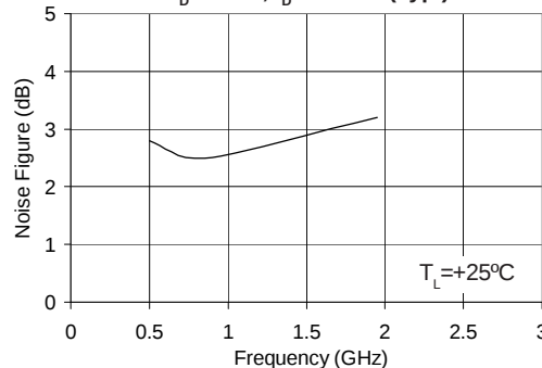
Noise Figure vs. Frequency V_D = 2.9\text{ V} , I_D = 35\text{ mA (Typ.)}
