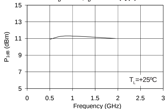
P_{1dB} vs. Frequency V_D = 2.9\text{ V} , I_D = 35\text{ mA (Typ.)}
