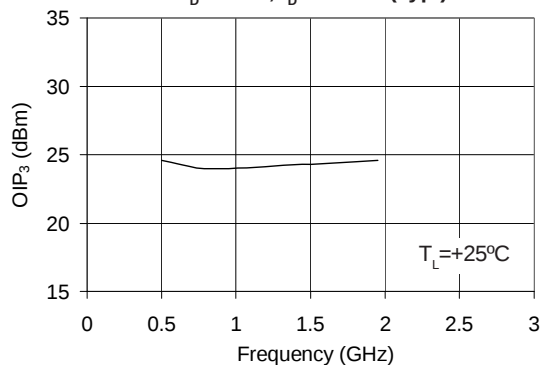
OIP_3 vs. Frequency V_D = 2.9\text{ V} , I_D = 35\text{ mA (Typ.)}
