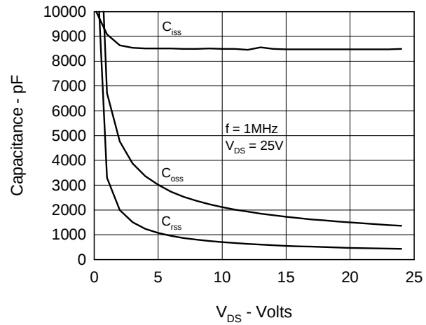
Fig.8 Capacitance Curves
