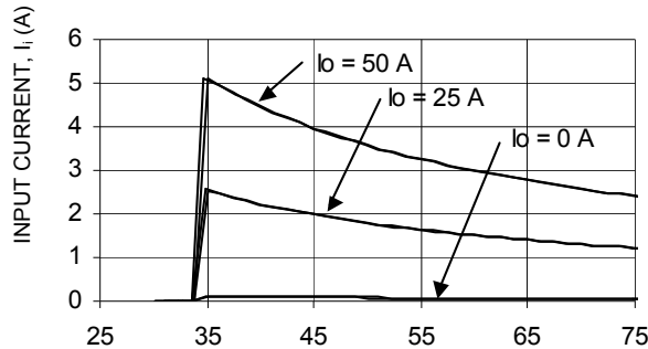
Figure 1. Typical Input Characteristic at Room Temperature.
