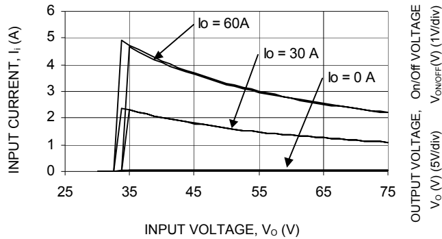
Figure 7. Typical Input Characteristic at Room Temperature.
