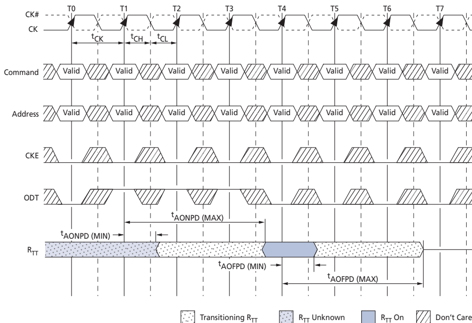
Figure 83: ODT Turn-Off Timings When Entering Power-Down Mode
