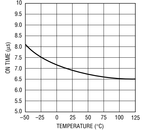
Switch ON Time
