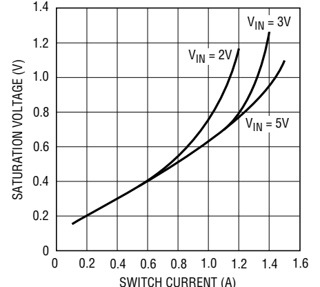
Saturation Voltage Step-Up Mode
