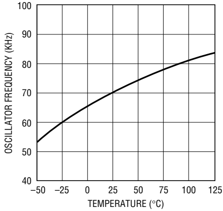
Oscillator Frequency
