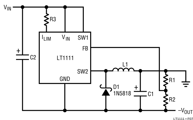
Figure 7. Positive-to-Negative Converter
