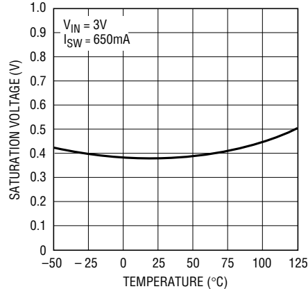
Saturation Voltage Step-Up Mode
