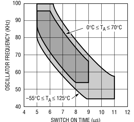
Minimum/Maximum Frequency vs ON Time
