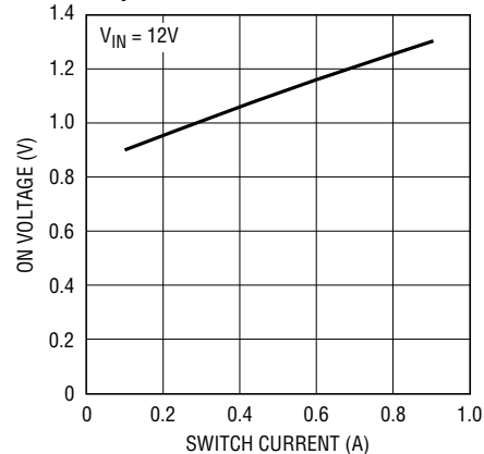
Switch ON Voltage Step-Down Mode
