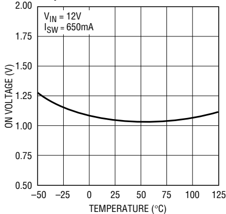
Switch ON Voltage Step-Down Mode
